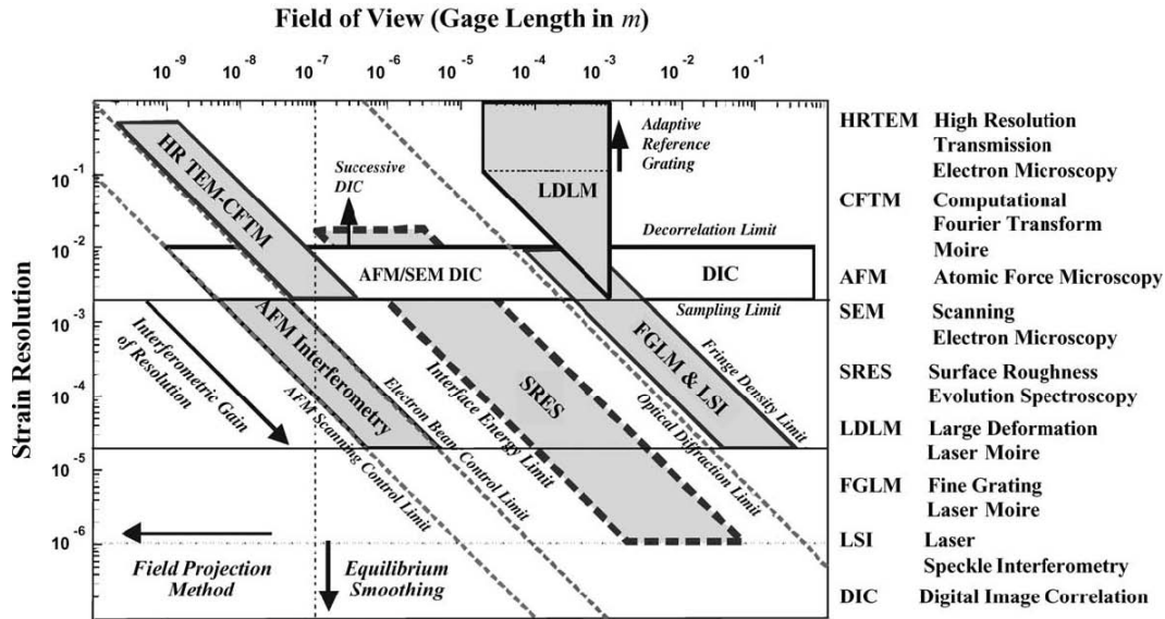
Fig. 1. Instruments and techniques for experimental micro and nano mechanics (courtesy of K.S. Kim of Brown University) where HRTEM, high resolution transmission electron microscopy; SRES, surface roughness evolution spectroscopy; CFTM, Computational fourier transform moire; FGLM, fine grating laser moir; AFM, atomic force microscopy; LSI, laser speckle interferometry; SEM, scanning electron microscopy; DIC, digital image correlation; LDLM, large deformation laser moire.
